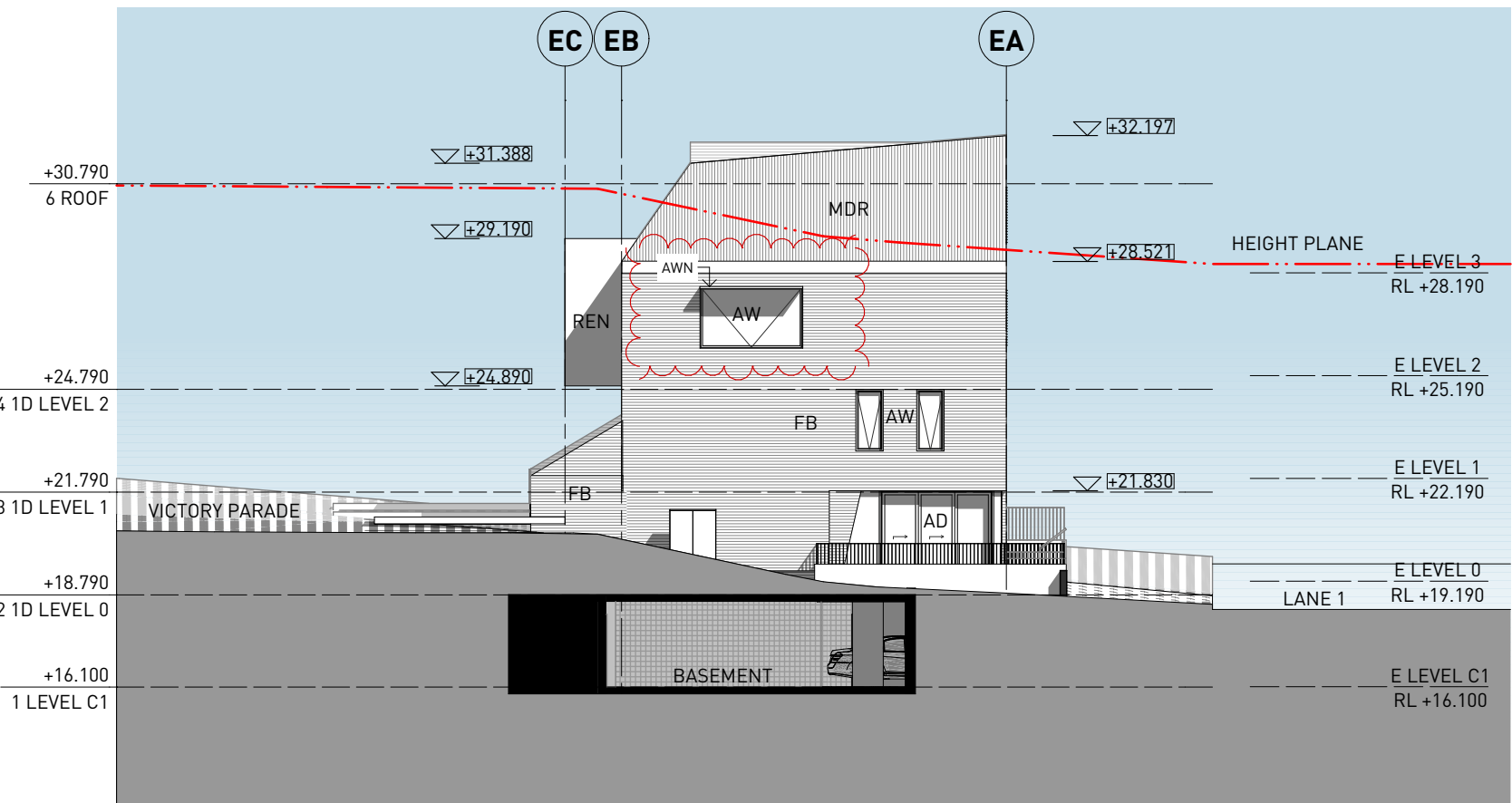
3 BUILDING E NORTH ELEVATION 1:200
