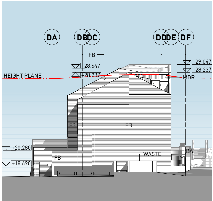
3 BUILDING D WEST ELEVATION 1:200
