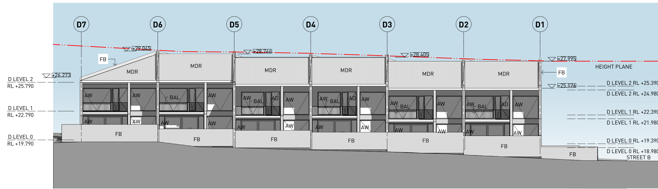
1 BUILDING D NORTH ELEVATION 1:200
