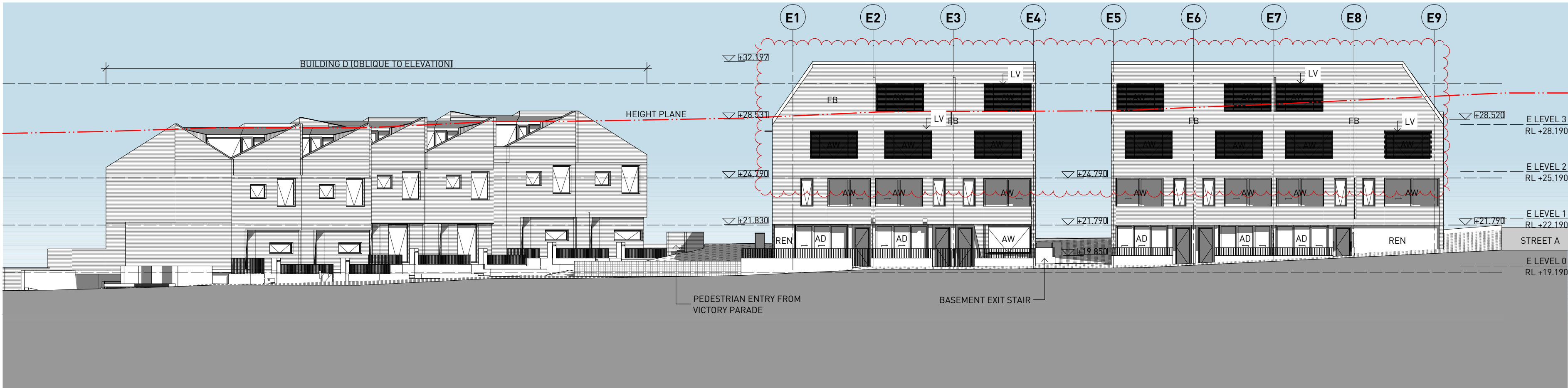
2 BUILDINGS D AND E WEST ELEVATION 1:200
