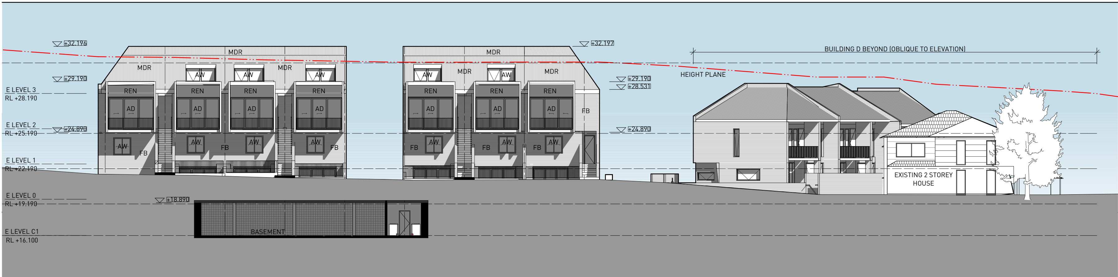
1 BUILDING D AND E EAST ELEVATION 1:200
