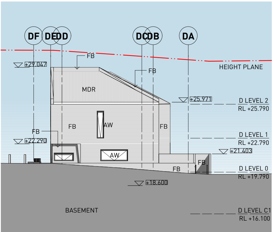
4 BUILDING D EAST ELEVATION 1:200
